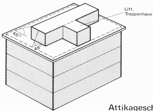
Attikageschoss
